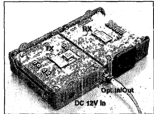
Fig. 4 Internal view of wireless Gigabit Ethernet transceiver.
