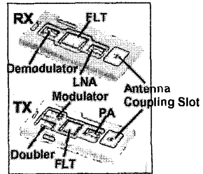
Fig. 3 Transmitter and receiver MCM's photograph.
