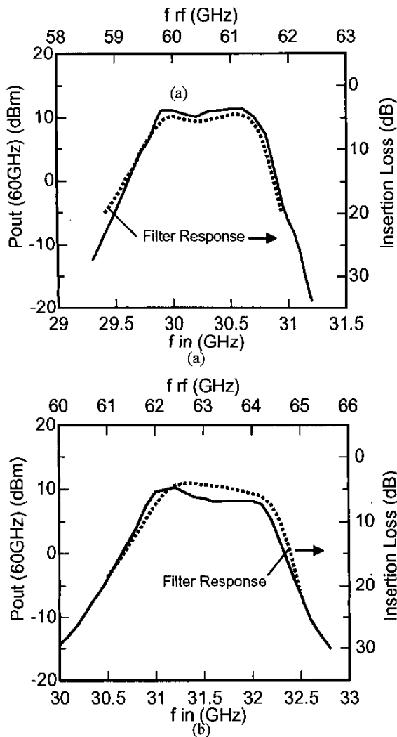
Fig. 5 Frequency response of peak output power for TX MCM. (a) f1 of 60.3GHz, (b) f2 of 63.13GHz.
