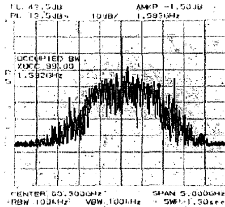
Fig. 9 Transmitter output spectrum for 1.25Gbps data input. (Center : 60.3GHz, Span : 5GHz)
