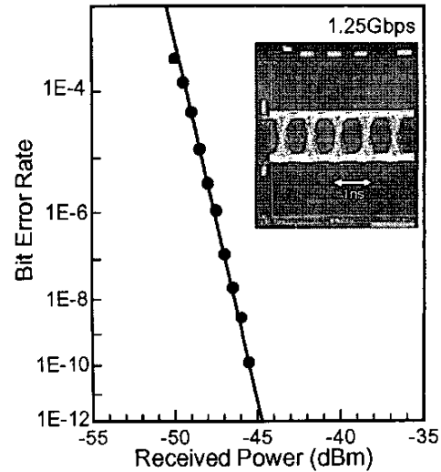
Fig. 6 Bit error rate performance and eye pattern for receiver.
